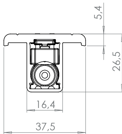
DETAIL J SCALE 1 : 1
