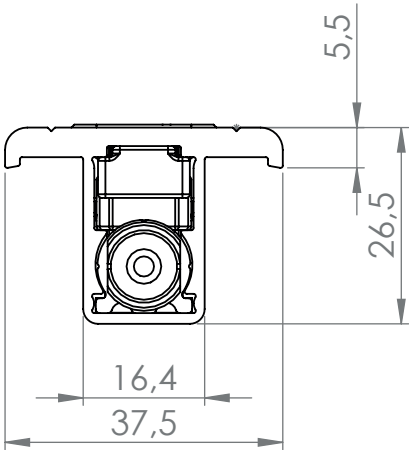
DETAIL AM SCALE 1 : 1
